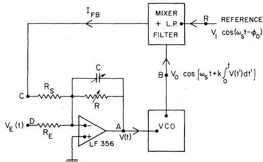
FIG. 14. Schematic diagram of the phase-locked loop used in our simulations. Typical circuit values are R = 11 \text{ k}\Omega , C = 100 \text{ nF} , k = 4\pi \times 10^3 \text{ s}^{-1}/\text{V} which lead to a natural frequency \Omega_0/2\pi = 600 \text{ Hz} and a Q = 4 . We also used R_E = R_S = 10 \text{ k}\Omega and a reference frequency \omega_s/2\pi = 100 \text{ kHz} .
